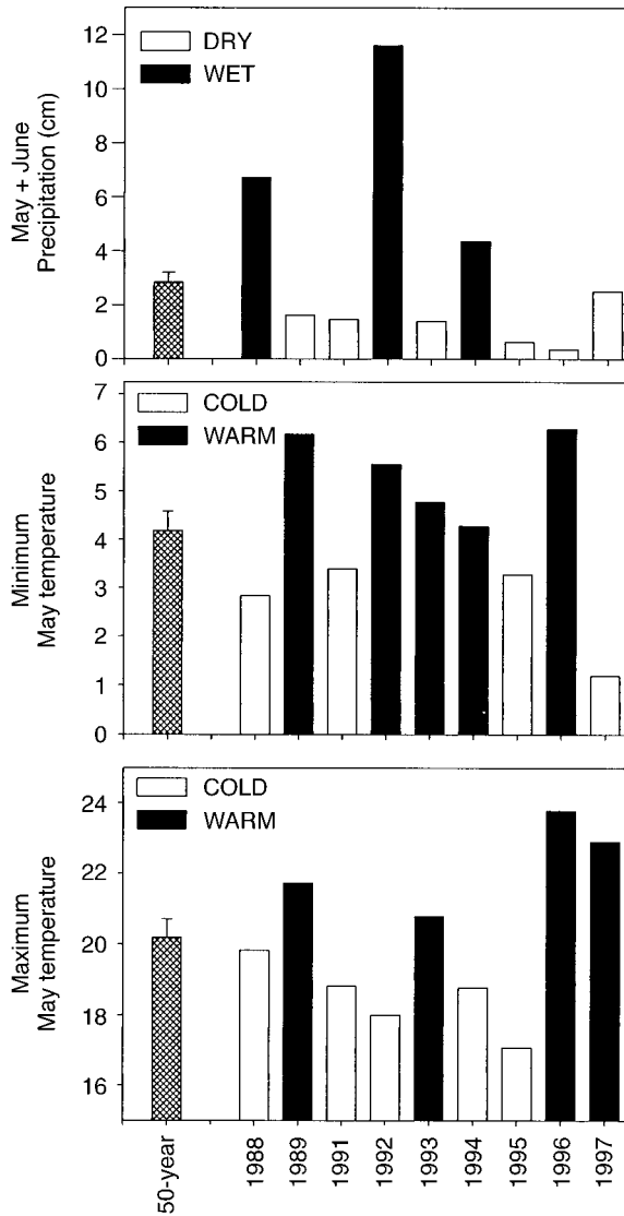
FIG. 3. Total precipitation during May and June (when >90% of nests of these species are initiated) for study years from 1988 to present; field data were not collected in 1990. Mean precipitation (+ 1 SE) over the previous 50 yr is provided for comparison to characterize wet and dry years. Note that wet and dry years alternate regularly across the nine study years and included the wettest (1992) year on record and one of the driest (1996).
