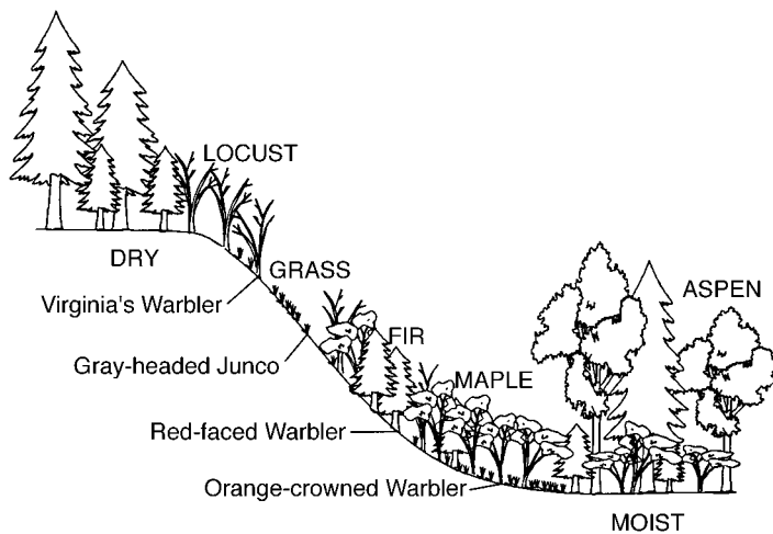
FIG. 1. Characterization of a vegetation gradient for forest drainages in Arizona. New Mexican locust ( Robinia neomexicana ) is xeric tolerant and was more abundant at the top than in the bottom of drainages (Martin 1998). Canyon maple ( Acer grandidentatum ) is associated with mesic conditions and was more abundant in the bottom than at the top of drainages (Martin 1998). Small (<3 m in height) firs ( Abies concolor , Pseudotsuga menziesii ) were similar in abundance over the entire gradient. The four ground-nesting bird species that coexist in these drainages exhibit clear nest site preferences that differ across this microclimate/vegetation gradient (Martin 1996, 1998). In general, Virginia's Warblers prefer xeric microhabitats dominated by locust high on slopes. Gray-headed Juncos prefer open grassy sites with an abundance of locust, indicating a tendency toward xeric sites. Red-faced Warblers prefer more mesic sites dominated by small firs and maple relatively low on the slope, and Orange-crowned Warblers prefer mesic microhabitats dominated by maple low on the slope (Martin 1998).
