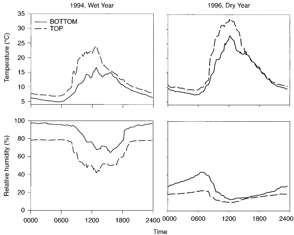
FIG. 2. Relative humidity and temperature were measured at the top and bottom of the slope at 30-s intervals and averaged over 5 min for 5-d moving averages in late May 1994 and 1996. Probes for measuring microclimate were placed in the same permanent sites each year to control any site effects. Probes at the top were placed near the ground in a locust patch typical of Virginia's Warblers, and probes at the bottom were placed in a maple patch typical of Orange-crowned Warblers (see Fig. 1; Martin 1998).
