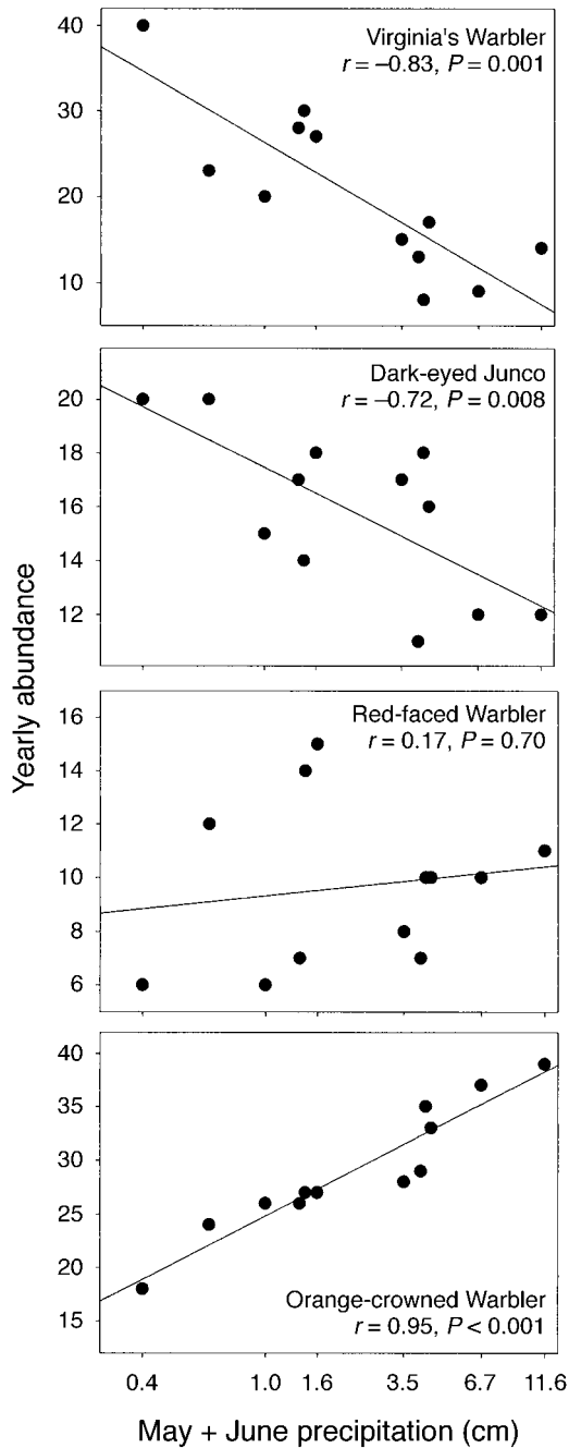
FIG. 9. Correlations of yearly abundance (obtained based on summed counts over 10 study plots studied since 1985) with May and June precipitation for each of the four species over 12 years (from 1985 to 1997).
