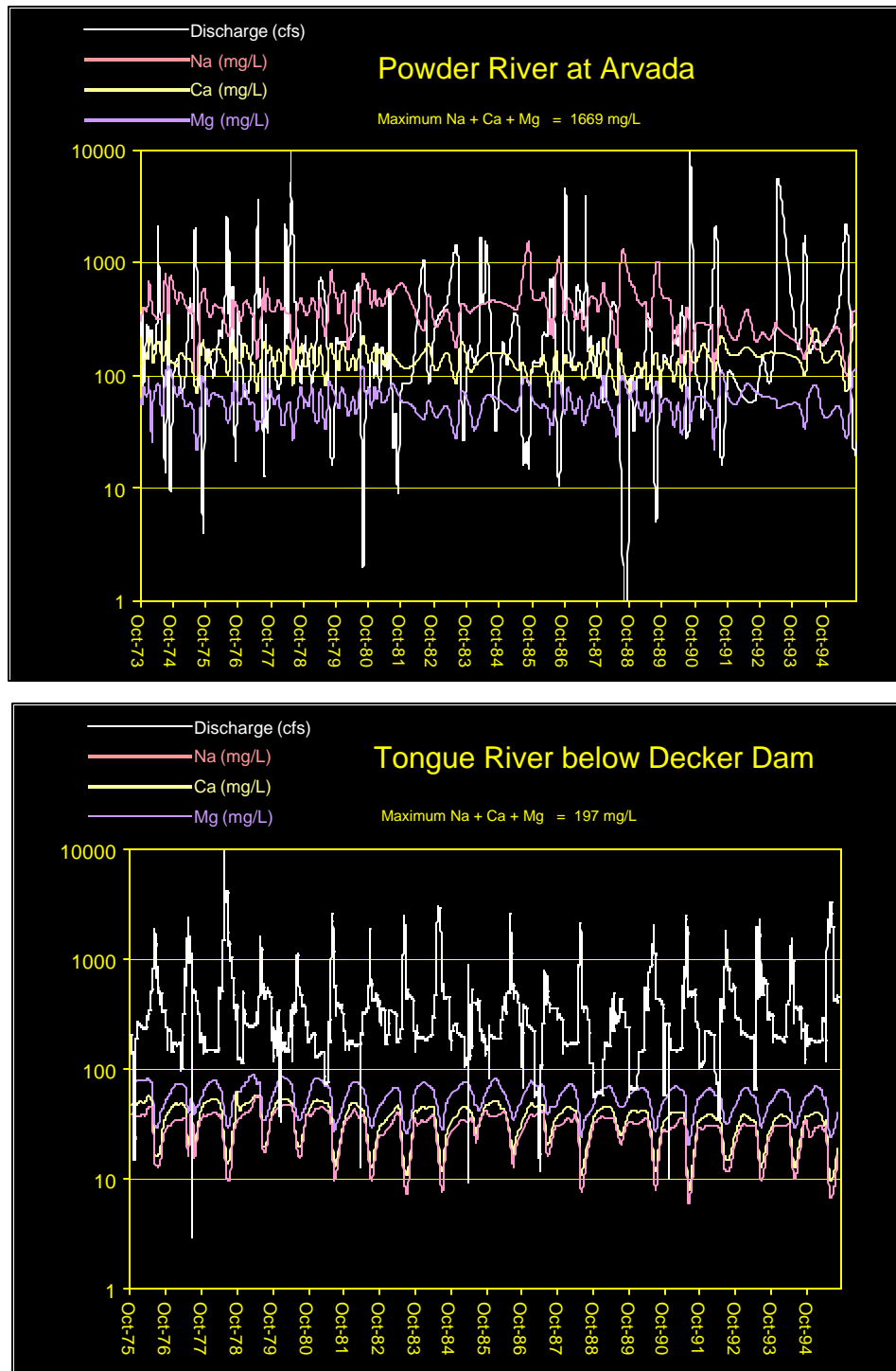
Figure 1. Discharge (cubic feet per second) and Sodium (Na), Calcium (Ca) and Magnesium (Mg) concentrations (mg/liter) in the Powder River at Arvada, Wyoming and in the Tongue River below Decker Dam near Decker, Montana, during the two decades preceding coalbed methane development in either Wyoming or Montana.
