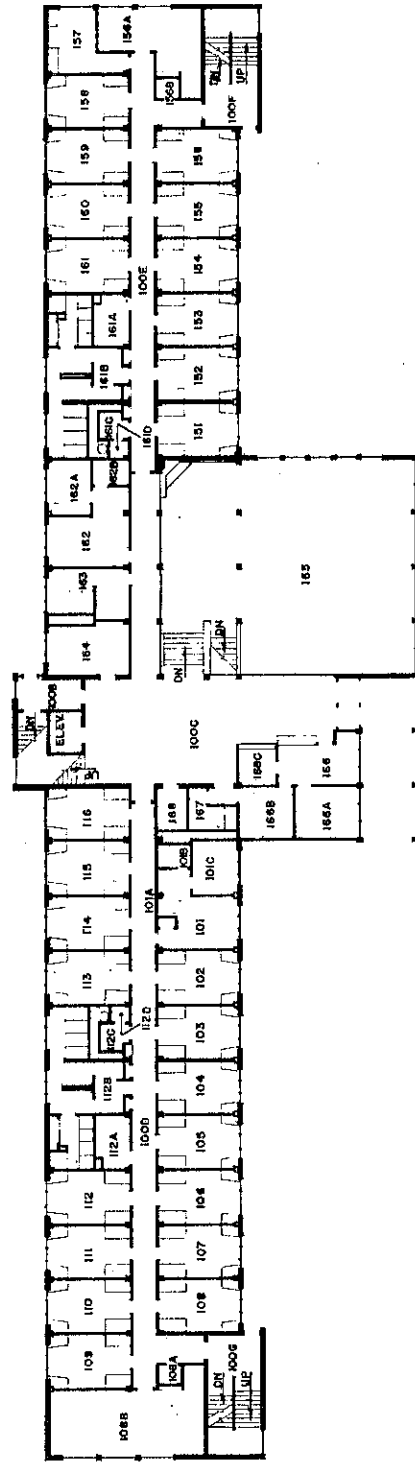
FIRST FLOOR
