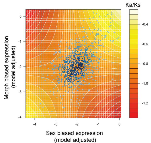
Figure 4. Effects of morph-biased and sex-biased expression on Ka/Ks in horned beetles. Contour plots of the effects of morph-biased expression and sex-biased expression on Ka/Ks in O. taurus vs O. nigriventris (A) and O. taurus vs T. dichotomus (B) comparisons. The contours are predicted from the general linear models given in Table 6. Super-imposed (blue dots) are the model adjusted values for sex-biased expression and morph-biased expression. These represent the averaged differences in gene expression between sexes and between horned- and horn-less males. These were previously calculated in [28]. Sex-biased expression, morph-biased expression and Ka/Ks have been log-transformed. doi:10.1371/journal.pone.0088364.g004
