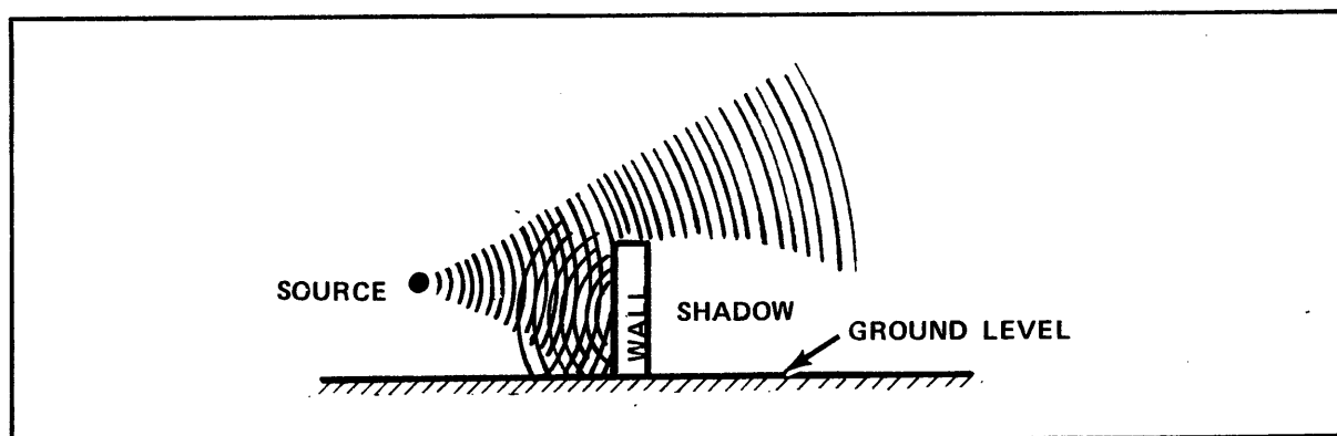
Figure 6. Diffraction barrier effects.
