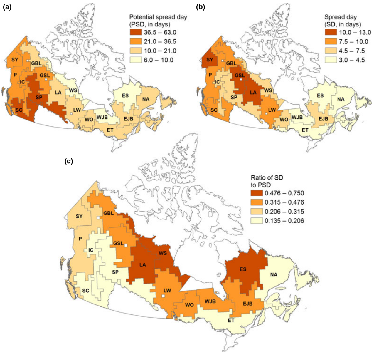
Fig. 4 Potential and realized fire spread across Canada. The median values of the frequency distributions of the potential spread days (PSD) (a) and spread days (SD) (b), as well as the ratio of medians of the distributions of SD and PSD by fire zone. A high ratio (i.e., closer to 1) indicates high realized fire spread relative to the potential fire spread.
