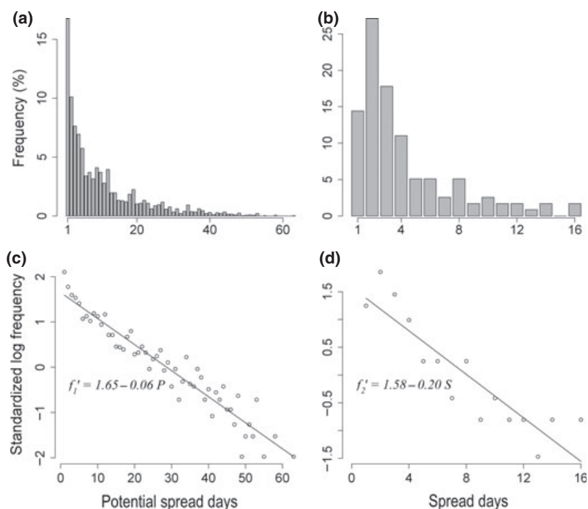
Fig. 3 An example of the frequency distribution of potential spread days (PSD) (a) and spread days (b), as well as the linear regression fit between the log-transformed frequency and PSD (c) and SD (d) for the Pacific zone.
