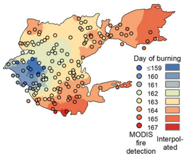
Fig. 2 Example of daily fire progression used to compile spread days. The daily MODIS fire detections (Julian day) (dots) are interpolated (Parks, 2014) for each active day of spread within the perimeter of fires from the Canadian National Fire Database (see Methods).
