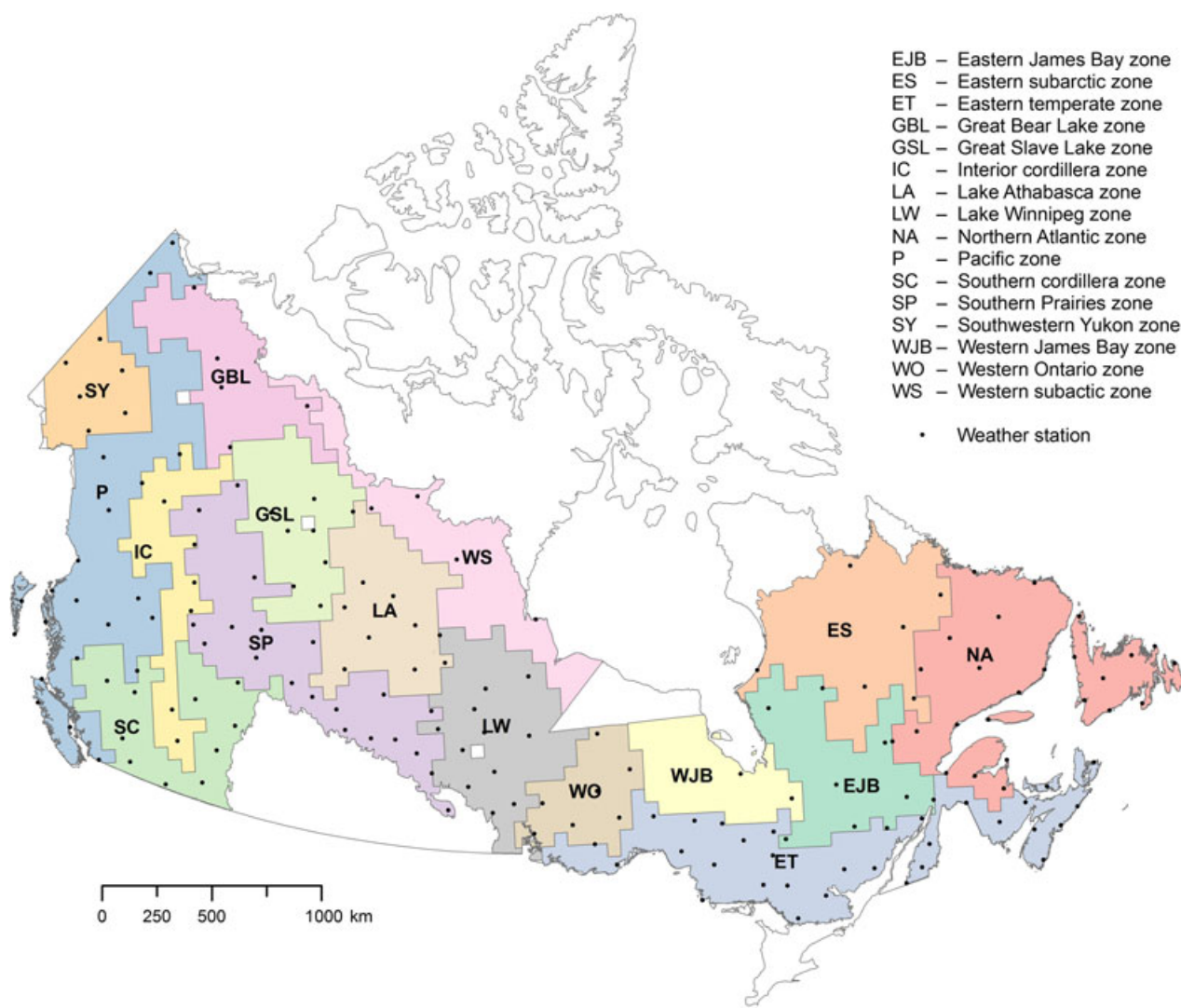
Fig. 1 The fire zones and Environment Canada weather stations (black dots) used in this study. Medians from distributions of potential spread days and spread days were computed on the basis of each zone.
