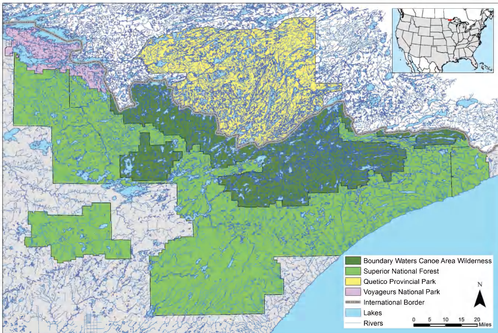
Figure 1—The BWCAW and surrounding protected areas.
