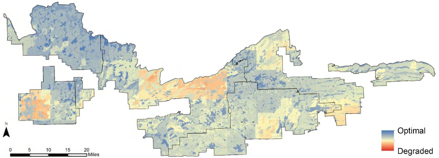
Figure 7—Map of the natural quality of wilderness character. Blue depicts optimal condition and red depicts degraded condition.
