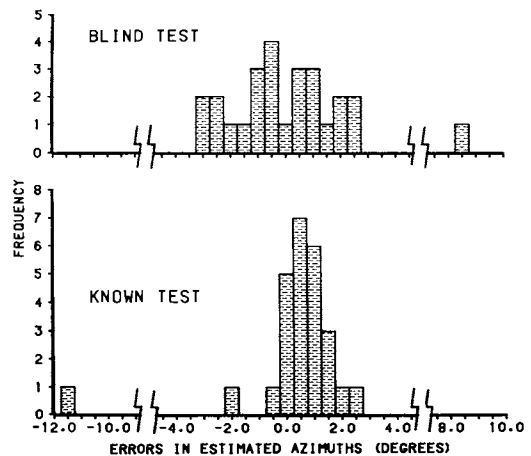
Fig. 1. Frequency histogram of errors in estimated azimuths to radio transmitters using identical locations for known and blind accuracy tests.
